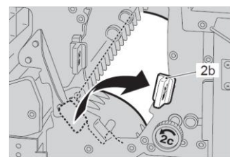
Paper Jam at the Lever 2a, 2b, 2c & 2d,
