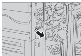
Paper Jam at the Lever 1a & 1b
